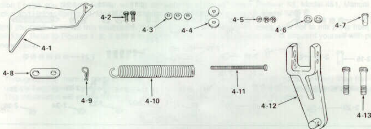
MANUAL LIFT BRACKET AND HELPER SPRING KIT 528
