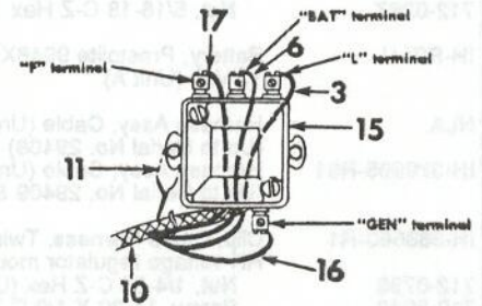
View of voltage regulator showing connections
