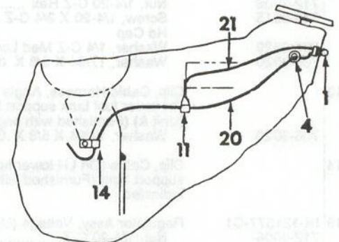
Left side view Tractors with retractable starter
