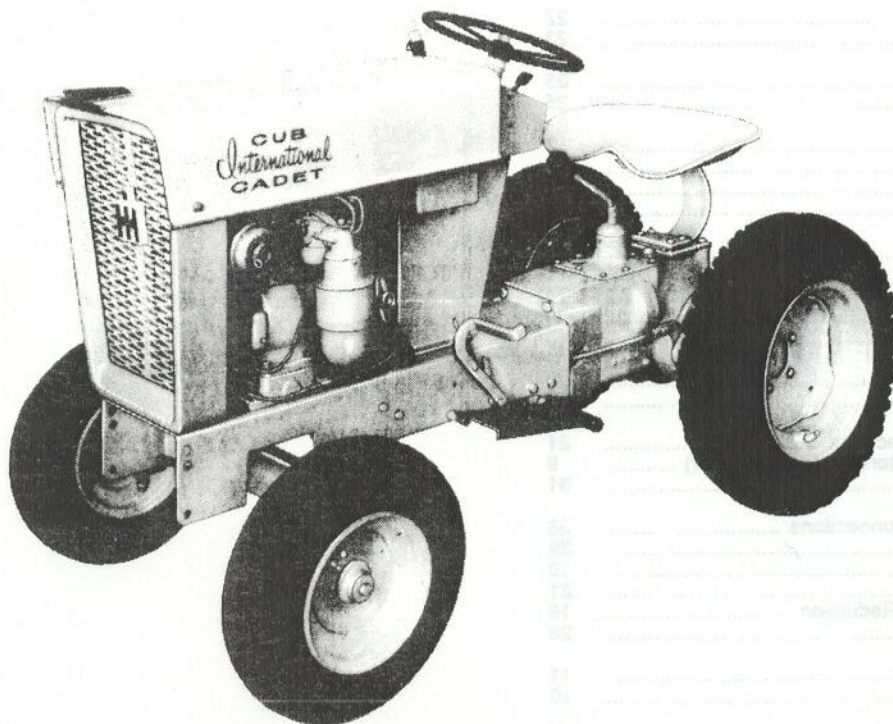
International Cub Cadet Tractor equipped with Retractable Starter (Left Front View)
